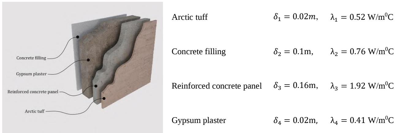
Fig. 2. 9 floor enclosing structure of a multi-story residential building
